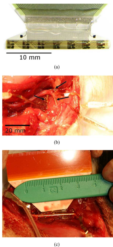
Fig. 1. (a) The matrix recording cuff before implantation (photo courtesy of Dr. Martin Schuettler, used with permission). (b) The tibial, peroneal, and sural nerves are exposed. Each has a stimulating cuff wrapped around it, indicated by an arrow. The sciatic nerve has been exposed but the recording cuff has not yet been placed. (c) The exposed sciatic nerve with the recording cuff wrapped around it.
