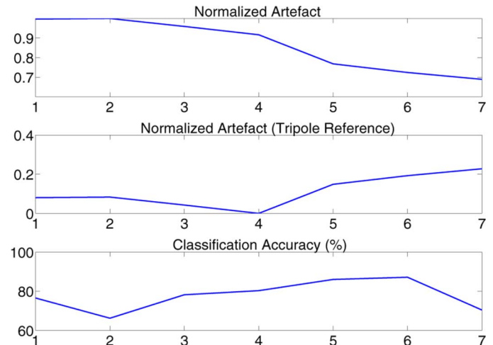
Fig. 8. Comparison of artefact variations and classification accuracy variations between contact rings in Rat 1. The top plot shows the normalized estimated variations of the stimulation artefact in the raw recordings, as a function of the contact ring. The middle plot shows the variations once the use of the tripole reference has been taken into account. The bottom plot shows the variations in the classification accuracy when each of the contact rings is used in turn. The middle and bottom plots are poorly correlated, arguing against the hypothesis that the stimulation artefact plays an important role in the classification accuracy.
