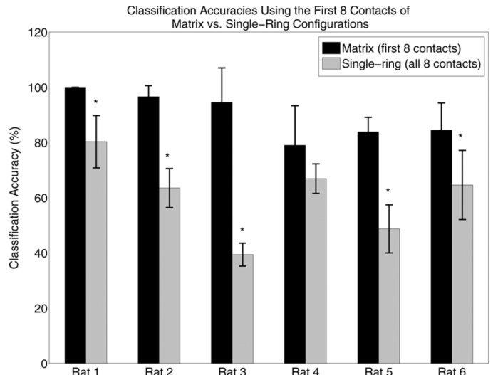
Fig. 5. Classification accuracy achieved with the first 8 selected contacts of the matrix and of the single-ring configurations, for each rat. The standard deviations shown are based on the set of 10 results obtained for each case during the 10-fold cross-validation process. The asterisk denotes a statistically significant difference ( p < 0.05 ).
