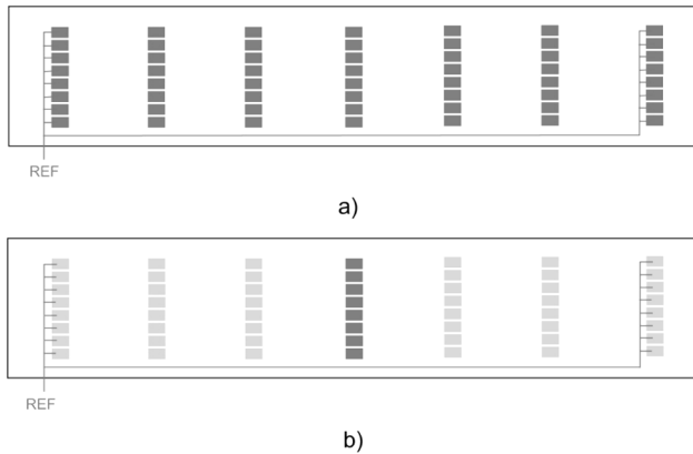
Fig. 2. Contact configurations for the matrix (a) and single-ring (b) cases. The contacts in dark gray are the ones that are available for use in the classification process. The contacts of the first and last ring are averaged to produce the reference, for both configuration.
